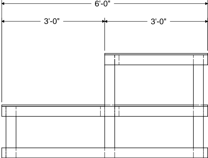
Dimensions do not include plywood
